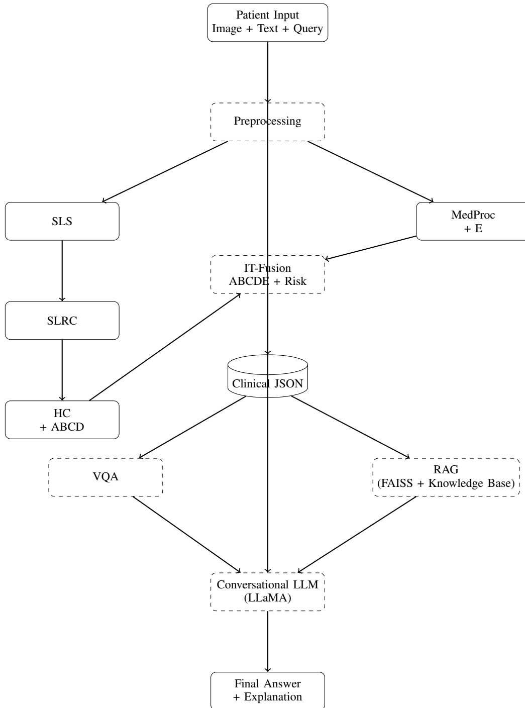
Fig. 1: NutriDermAI system architecture. Solid boxes denote implemented stages; dashed boxes denote planned future stages. The image pipeline (SLS → SLRC → HC) extracts ABCD features, while the clinical text pipeline (MedProc) derives the Evolution (E) score. Both streams converge in the IT-Fusion module, whose structured JSON output feeds the VQA and RAG layers before a LLaMA-based conversational LLM generates the final explainable response.
